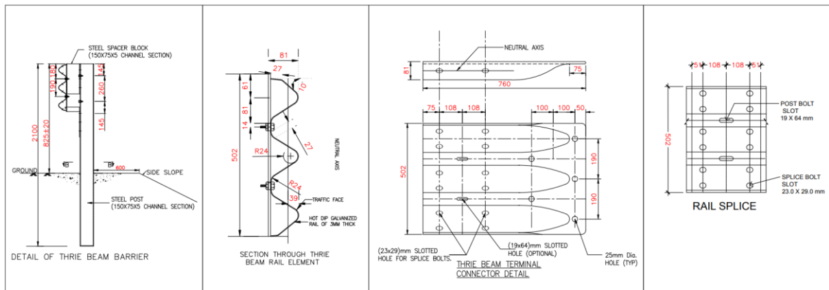
TYPICAL DETAILS OF THRIE BEAM STRUCTURAL ELEMENTS
